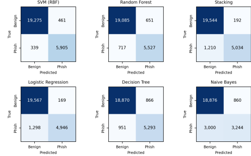
Fig. 1. Confusion matrices for the six classifiers on the domain-held-out test set.
